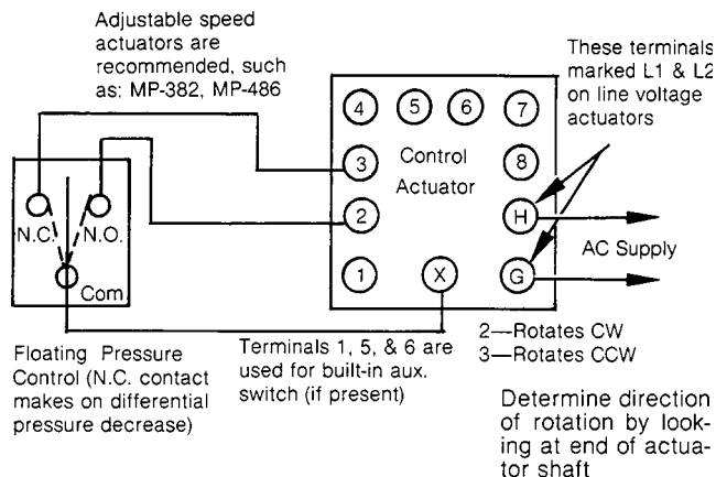
Figure-1 Typical Wiring.
